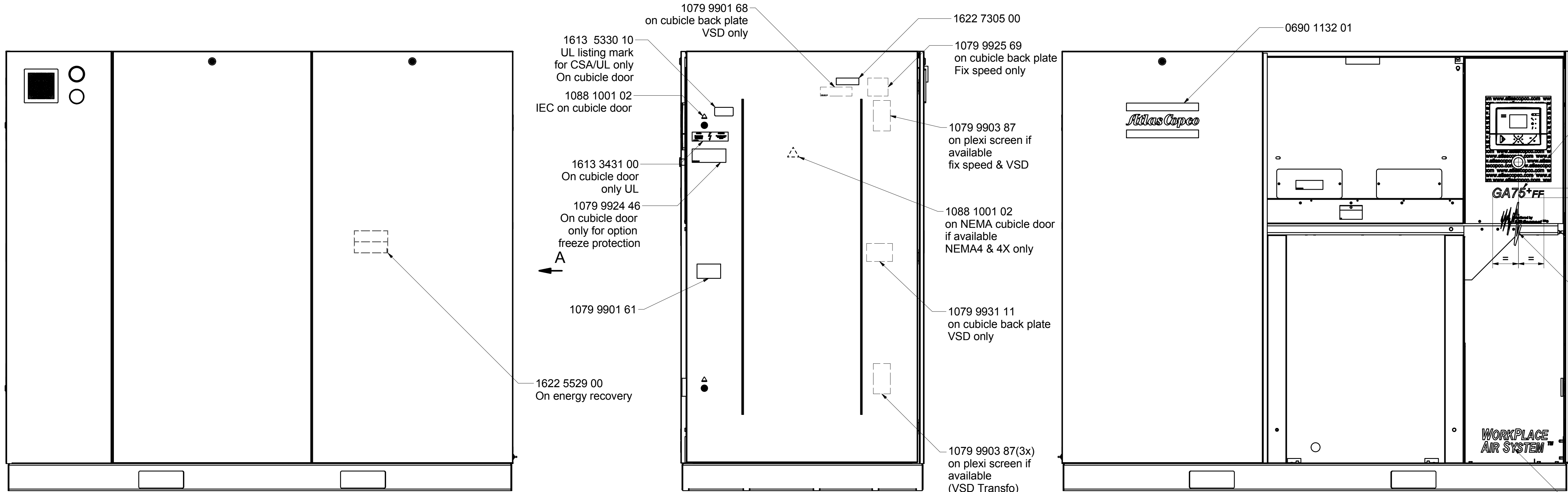
VIEW A
